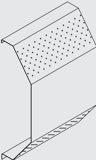
S-DSP5 - Double slope top, partial perforation
