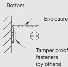
"AS" Removable enclosure section, interlocking style only, no joggles or joiners
