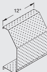
"AS" Removable enclosure section, interlocking style only, no joggles or joiners
