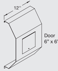
"AP" Access panel with access door, overlapping style only (w/allen key lock)
