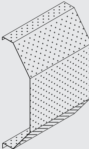
PDS5 - Double slope top, full perforation
