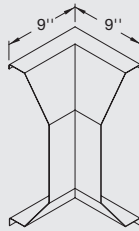
"IC" Inside corner
