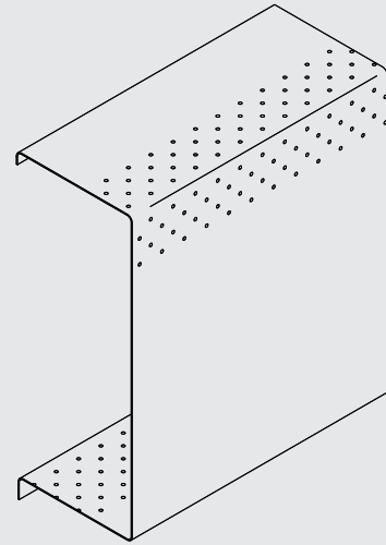
S-RP5 - Flat top, rounded outlet, partial perforation
