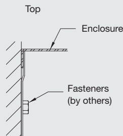
Offset mounting channel detail
