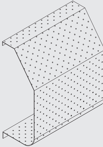
PS5 - Sloped top, full perforation
