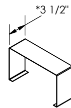
"WT" WALL TRIP STRIP *3-1/2", 5", 7-1/2"
