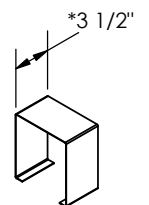
"WT" WALL TRIP STRIP *3-1/2", 5", 7-1/2"
